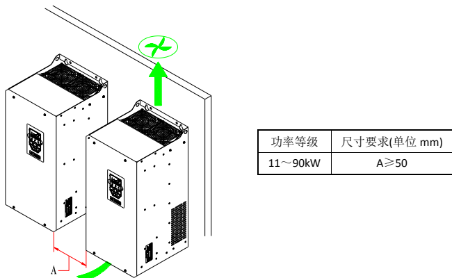
图3-3 Hope130G11T4~Hope130G90T4多台机器并排安装
