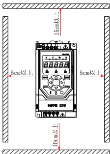
图3-1 单台机器（Hope130G0.75T4~Hope130G7.5T4）安装间隔
