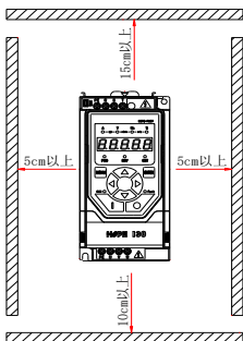
单台机器（Hope130G0.75T4~Hope130G7.5T4）安装间隔
