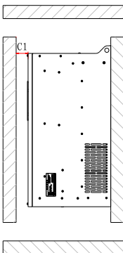
单台机器（Hope130G11T4~Hope130G160T4）安装间隔
