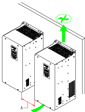
Hope130G11T4~Hope130G160T4多台机器并排安装
