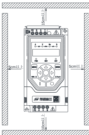
单台机器（Hope150PM0.75T4～Hope150PM7.5T4）安装间隔
