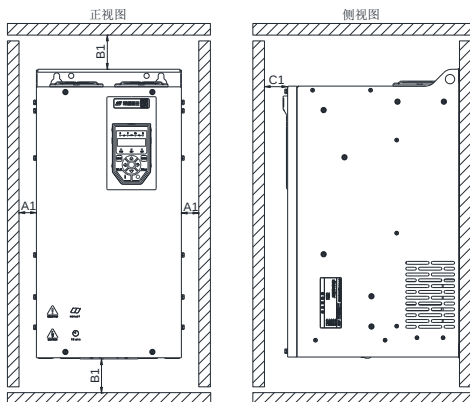
单台机器（Hope150PM11T4～Hope150PM160T4）安装间隔
