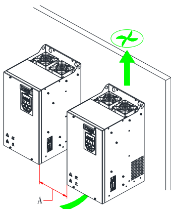
Hope150PM11T4~Hope150PM160T4多台机器并排安装
