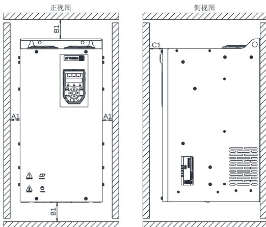
单台机器（Hope150G11T4~Hope150G160T4）安装间隔
