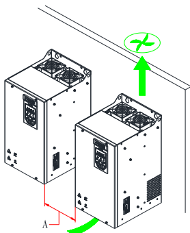
Hope150G11T4~Hope150G160T4多台机器并排安装
