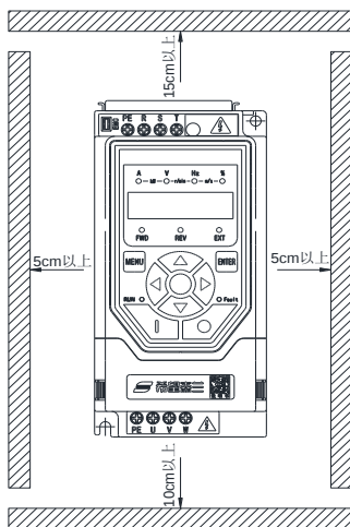
单台机器（Hope150G0.75T4~Hope150G7.5T4）安装间隔
