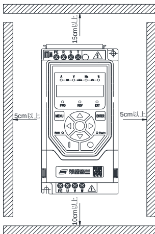
单台机器（Hope150PM0.75T4～Hope150PM7.5T4）安装间隔
